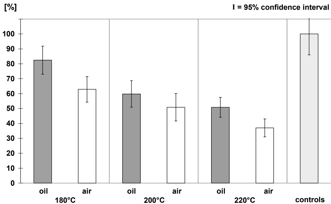
Fig. 4. Changes of the impact bending strength at Pinus sylvestris L. (150x10x10 mm 3 ) after treatment compared to untreated controls; n=15
