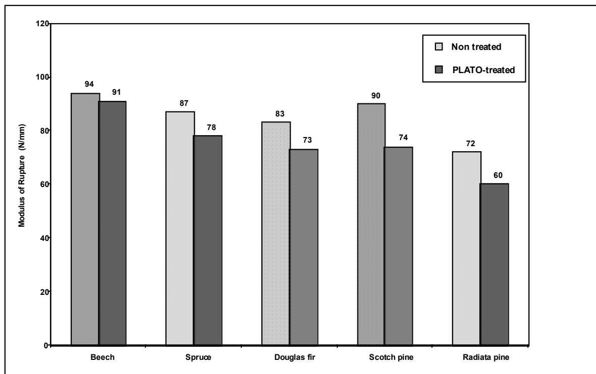
Figure 1. Modulus of rapture of some wood species before and after heat-treatment an whole black scale.
